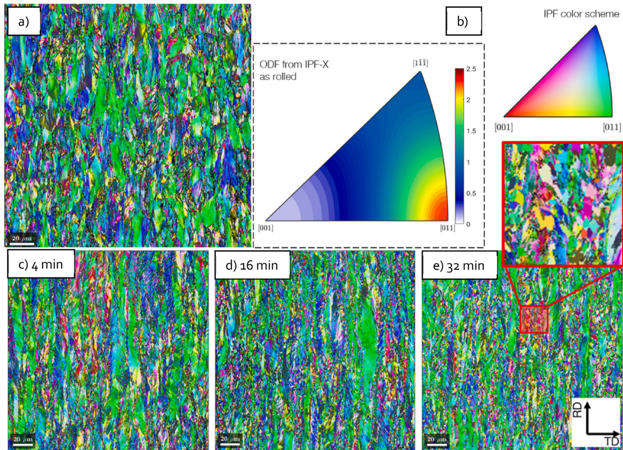
Fig. 4. EBSD IPF maps of the Fe–18Mn–0.3C steel (a) after warm rolling at 200 °C and after recovery annealing at 520 °C for (c) 4 min, (d) 16 min, and (e) 32 min with a magnified illustration of the already recrystallized grains. b) depicts the ODF from the given EBSD IPF-X map. Unassignable points are depicted as black.
